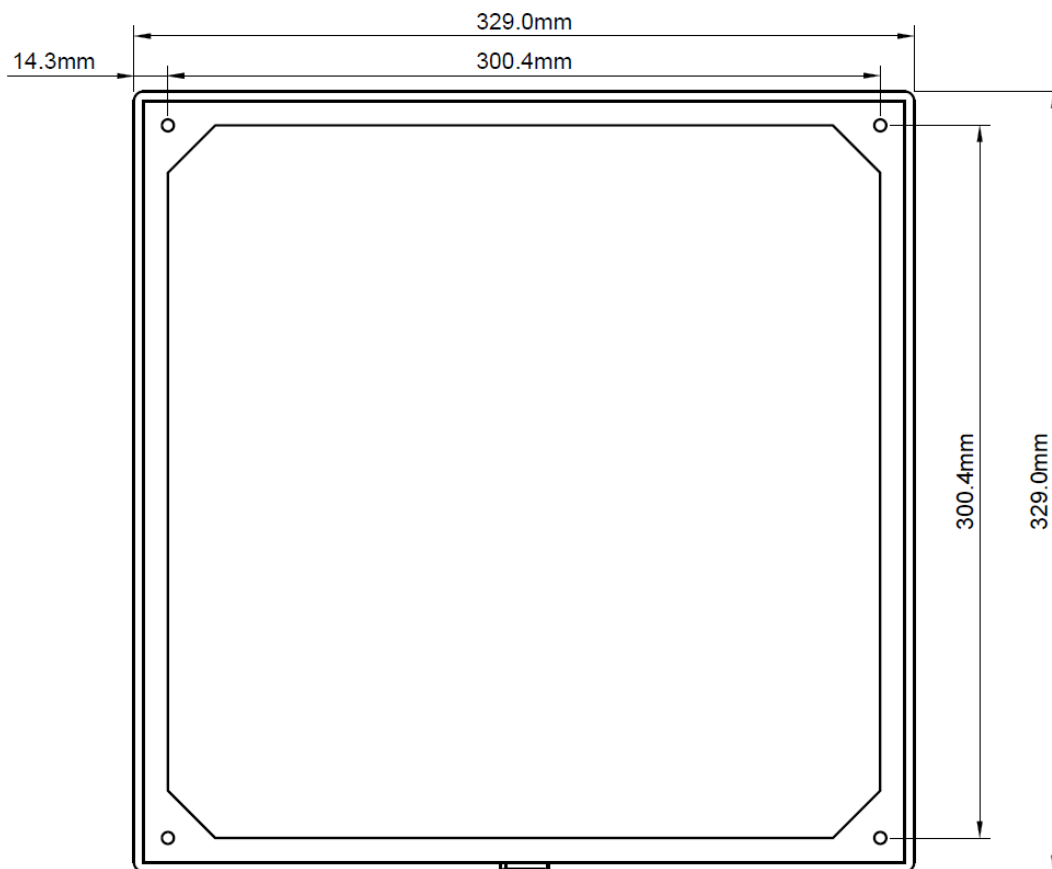
Picture 1: mounting holes
